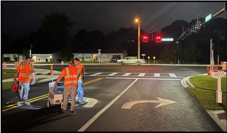
Placement of thermoplastic pavement markings
